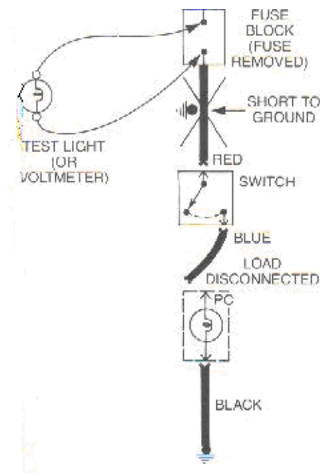
Fig.: Checking for Short
