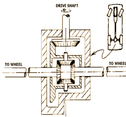
Fig 11: Differential section
