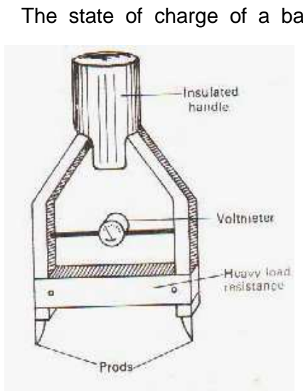
Fig.: High Rate Discharge Tester
