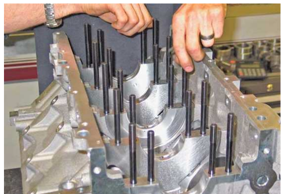
Fig-15 Main studs in engine block
