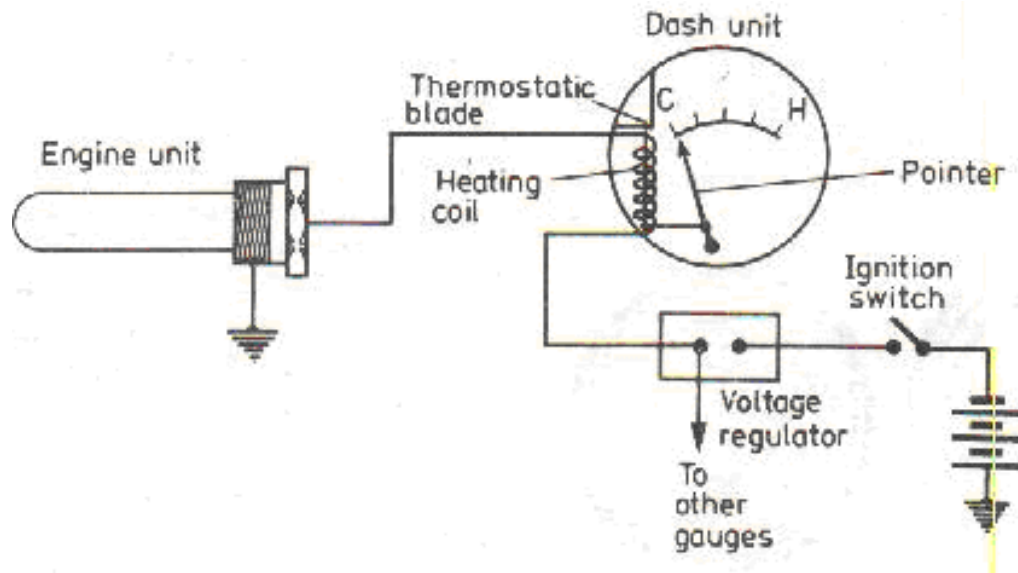
Fig.: Circuit of a Thermostatic Type Temperature Gauge
