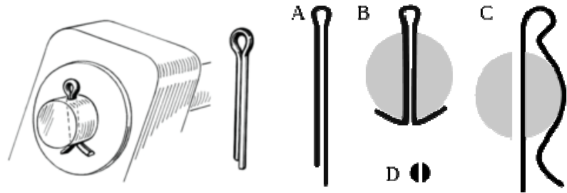
Fig-22 Split pin in shaft. A-new, B-installed, C-spring type, D-cross-section
