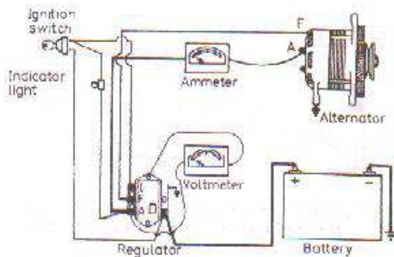
Fig.: Wiring Diagram for Testing Alternator and Regulator on the Vehicle
