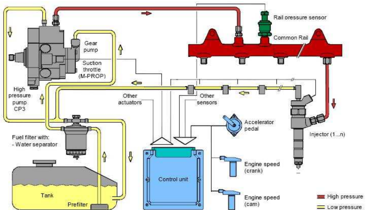
Fig 15 : CRDI System
