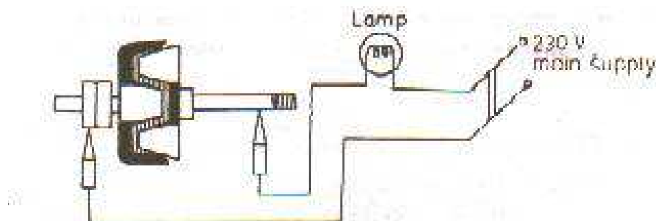
Fig. D: Circuit Diagram of Rotor Insulation test on Main Supply
