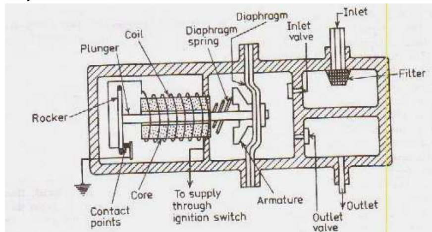
Fig.: Electric Fuel Pump (Diaphragm type)
