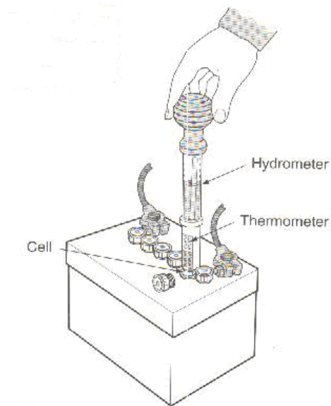
Fig.: Checking the Specific Gravity of Electrolyte with the help of Hydrometer.
