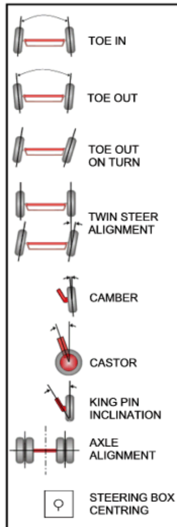
Fig14: Steering Angles
